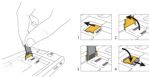
Figure 10. Insert the media card
