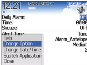
Figure 7. Full menu
