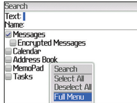
Figure 8. Short menu
